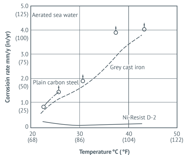
Figure 7 Corrosion in aerated seawater as a function of temperature
