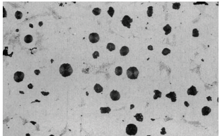
Figure 2 Typical Microstructure of Spheroidal Graphite Ni-Resist Alloys – Ni-Resist D-2W – Graphite Spheres and Carbide Areas within Austenite Matrix
