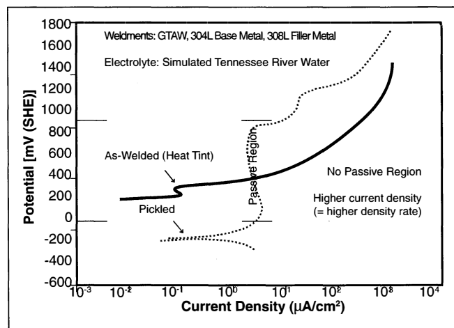
Figure 8 Polarization data showing effects of heat tint on corrosion resistance.
