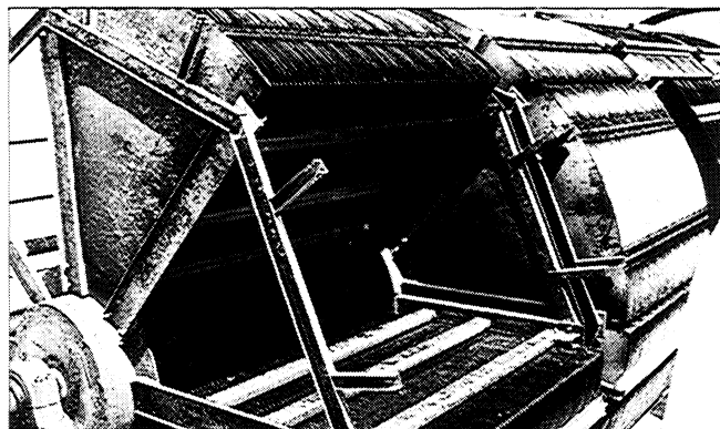
Figure 3 Type 409 stainless steel Rotating Biological Contractor (RBC) disassembled with MIC attack on arms.
