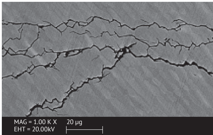
Figure 5 SEM micrograph showing cracking on S32750 specimens after 24 hours in 45% MgCl 2 at 155°C
