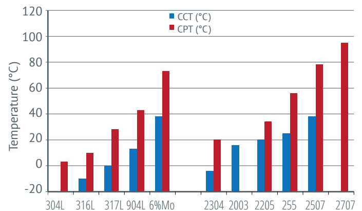
Figure 3 Critical pitting and critical crevice corrosion temperatures for various duplex and austenitic stainless steel. Measurements made using ASTM G48 Test methods A and B (results from reference (2) and producers' data).
