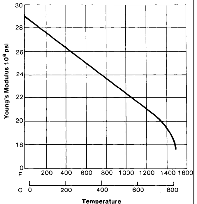
Figure 27 Tensile Modulus for Austenitic Stainless Steels (10)
